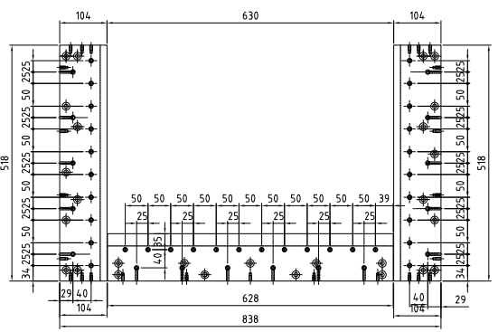
Worktable Hole Layout
