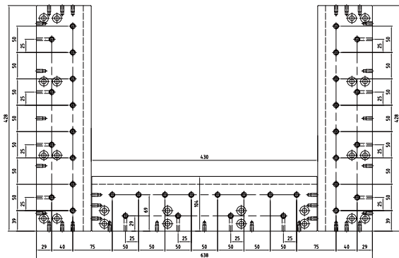
Worktable Hole Layout
