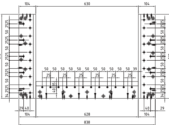
Worktable Hole Layout
