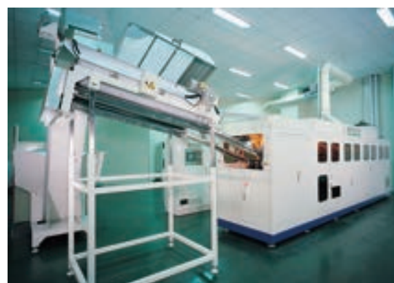
PET耐熱結晶瓶一結晶線 High-Speed Preform Crystallizing Machine
